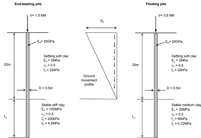
Fig. 5. End-bearing and floating pile in two-layer soil system
