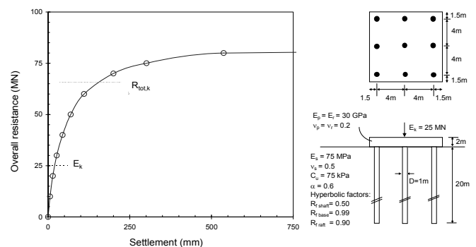
Figure 5. Load-settlement response and piled raft analysed
