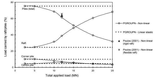
Figure 4. Load sharing between raft and piles
