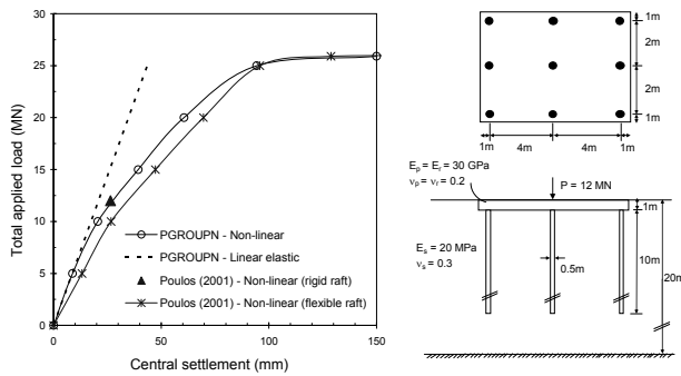
Figure 3. Load-settlement response and piled raft analysed
