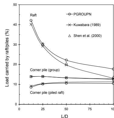
Figure 2. Load sharing between raft and piles
