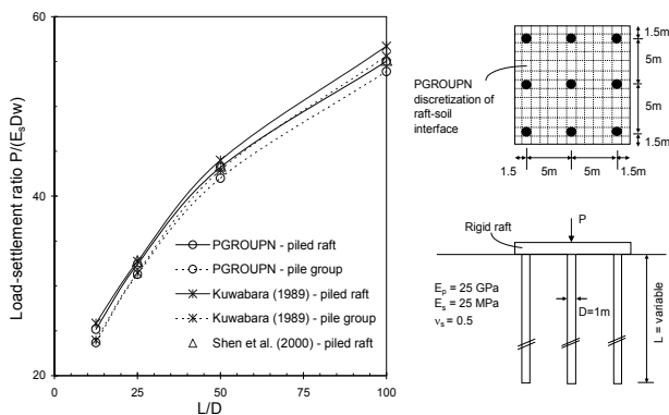
Figure 1. Load-settlement ratio and piled raft analysed
